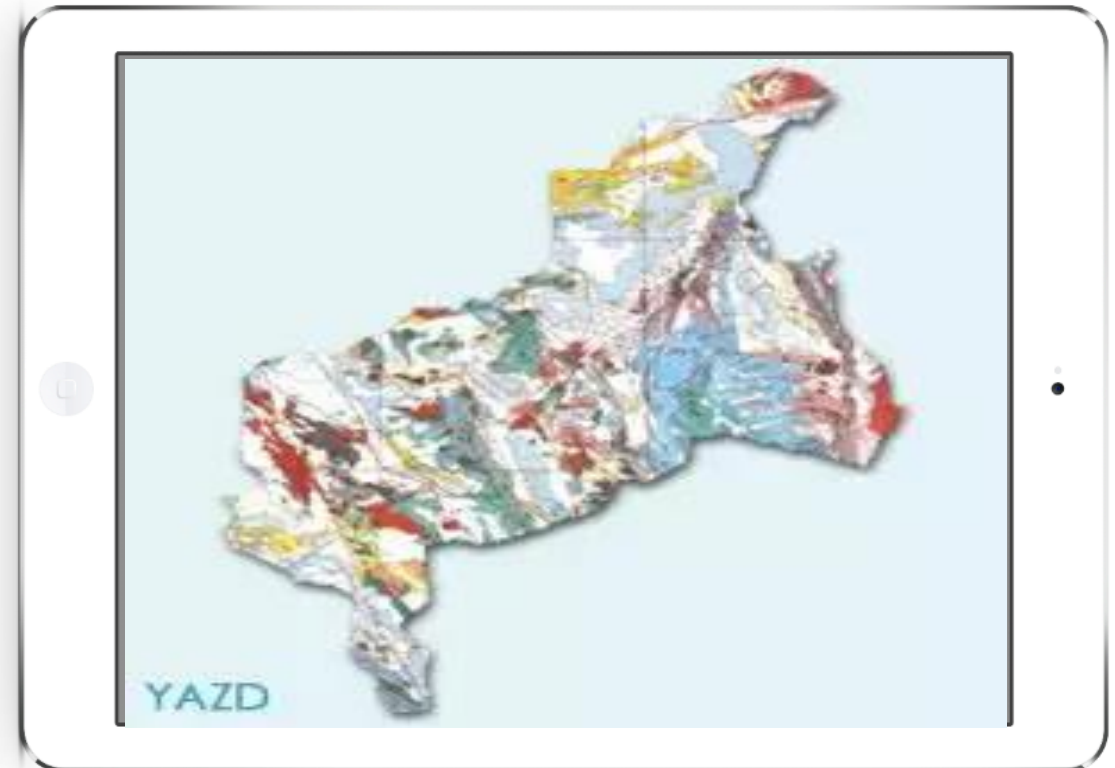
Mineral map , Yazd Province
